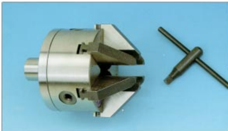
▲ Four-inch universal six-jaw chuck for workhead. No. 02
