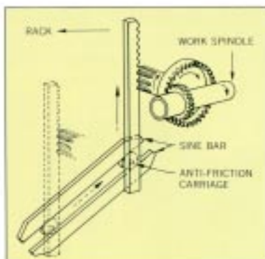
Spiral mechanism generates infinitely variable leads.
